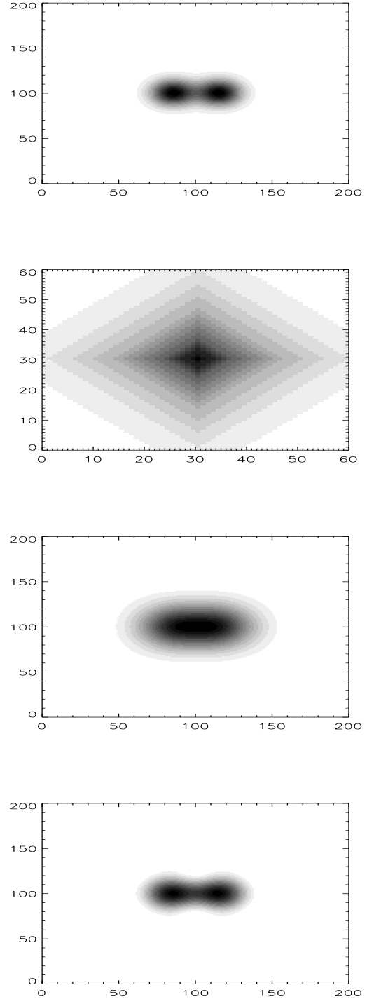
Figure 1. Example of deconvolution by shapelet decomposition: (a) Image before smearing, (b) Convolving kernel (PSF), (c) Smeared image, (d) Recovered image from the shapelet matrix inversion.
