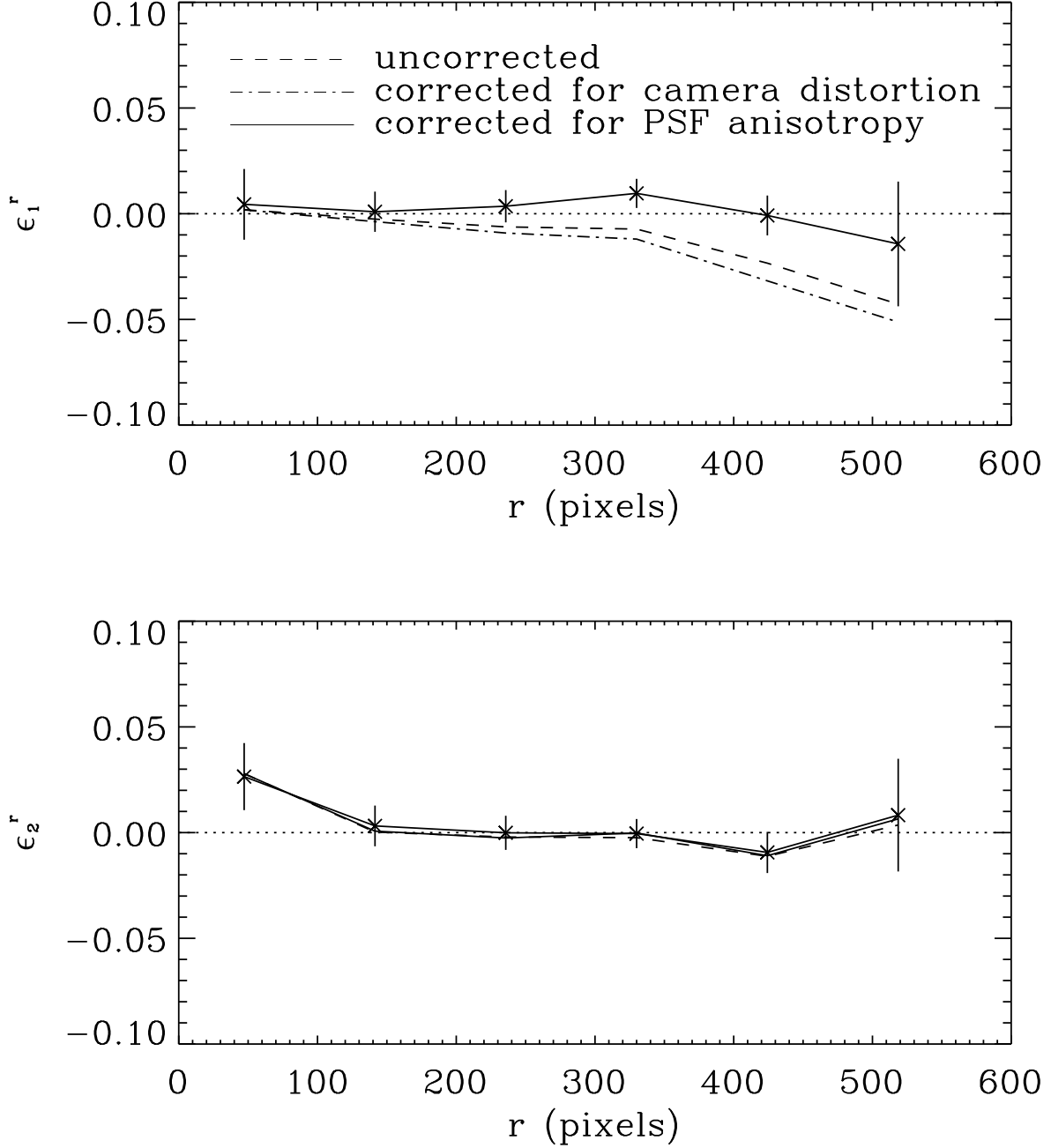
Fig. 13.— Effect of the corrections for small galaxies ( 1.0 < d' < 1.5 pixels, I < 26 ) in the survey strip. The profile for the galaxies is shown at different stages of the correction algorithm. The error bars are similar for each of the three profiles, but, for clarity, were only displayed for the last case.
