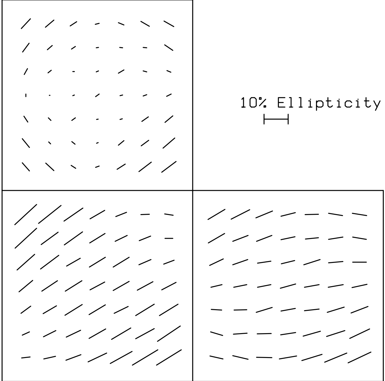
Fig. 4.— PSF ellipticity predicted by Tiny Tim. This figure corresponds to a focus of -1.5\mu\text{m} , close to the mean value for the Survey Strip observations. The ellipticities are shown after application of the camera distortion.
