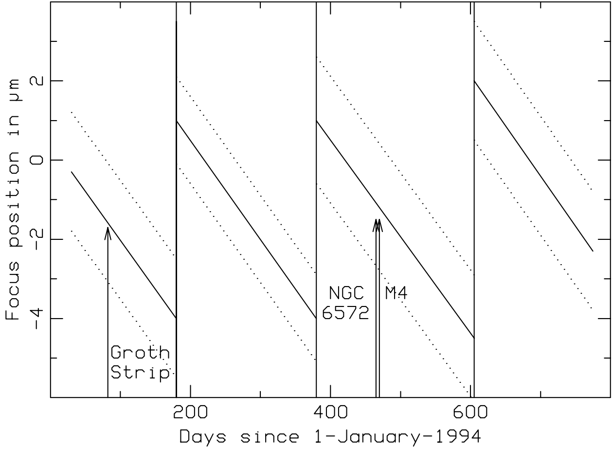
Fig. 5.— HST focus as a function of time. The vertical lines give the times of mirror movements generated to bring the telescope back into focus. The diagonal lines represent the average mirror position as a function of time. Orbit-to-orbit “breathing” produces considerable variations (up to several microns) about these mean values. The rms value of these variations is shown by the dotted lines. This figure is patterned after Figure 5.7 in Biretta (1996). The values corresponding to the observations of the Survey Strip, and of the M4 and NGC6572 globular clusters are also indicated.
