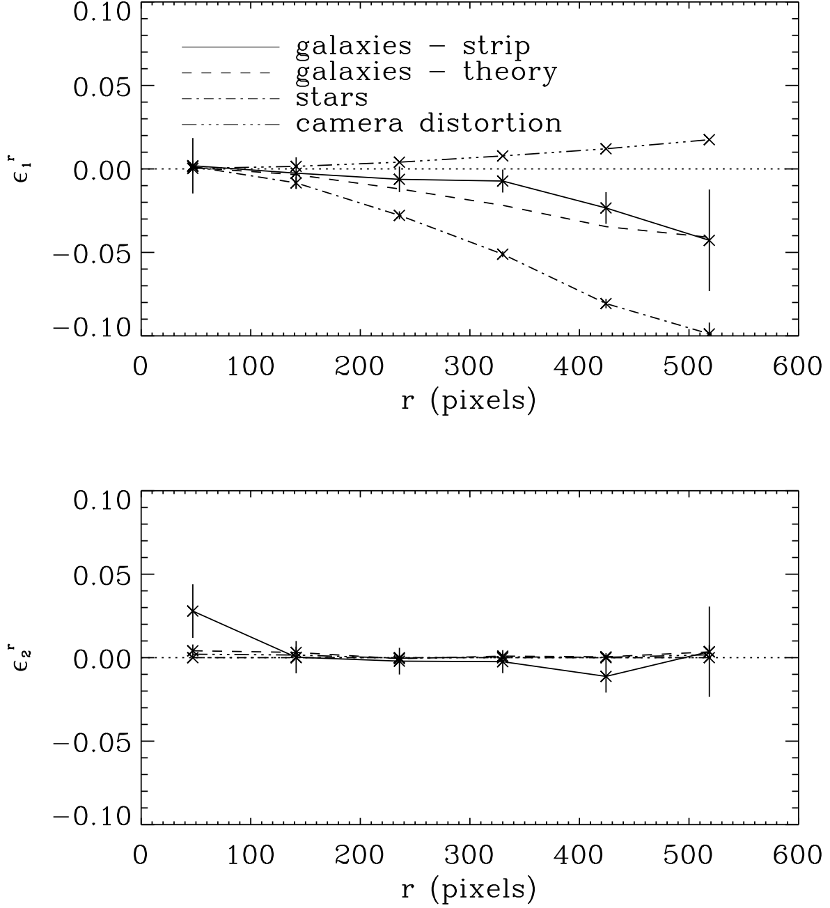
Fig. 11.— Rotated ellipticity profile for small galaxies in the survey strip. Galaxies were selected to have I < 26 , and radii 1.0 < d' < 1.5 pixels. The PSF and the camera distortion ellipticity \epsilon_i^{\phi,r} is also shown for comparison. The profile for the Strip galaxies expected in the simplified theoretical model is also shown (see text).
