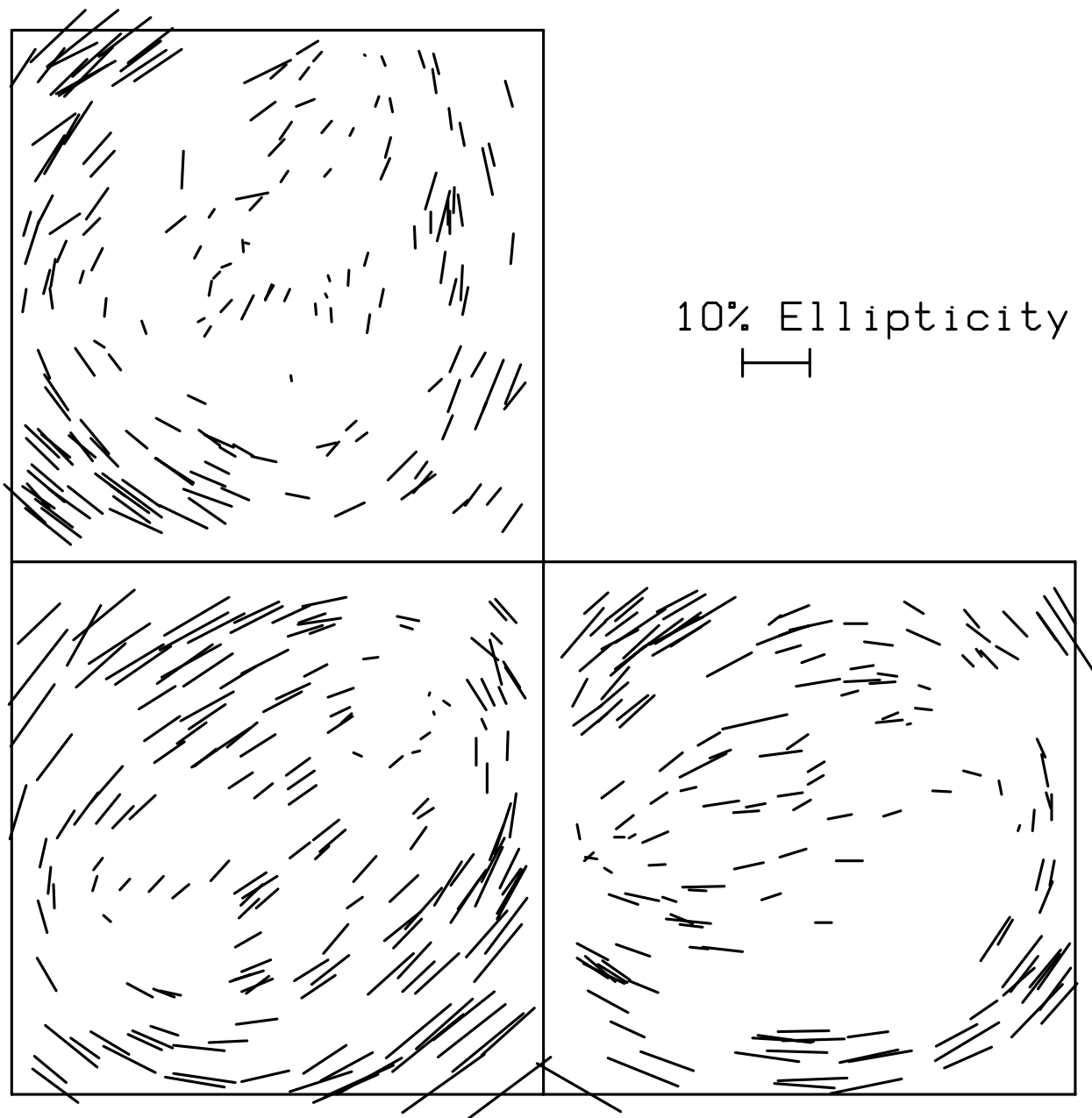
Fig. 8.— Ellipticities of the stars in the globular cluster M4. A Gaussian weight function of width \omega_* = 2 pixels was used to measure the stellar moments.
