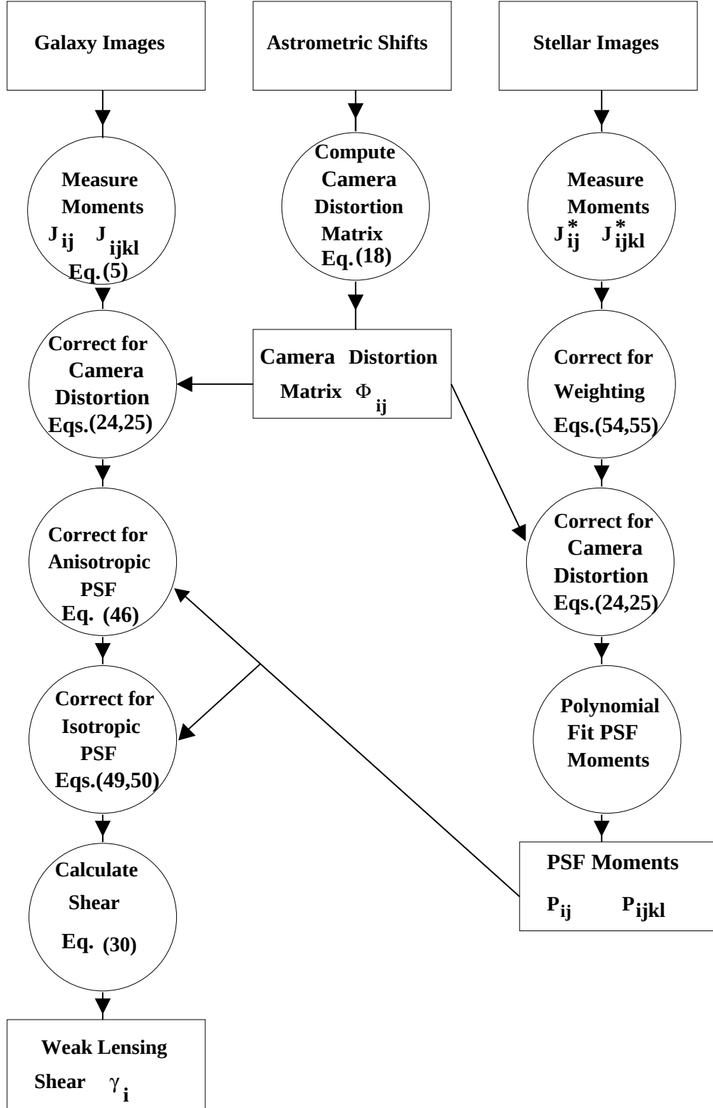
Fig. 1.— Synopsis of the weak lensing measurement method.
