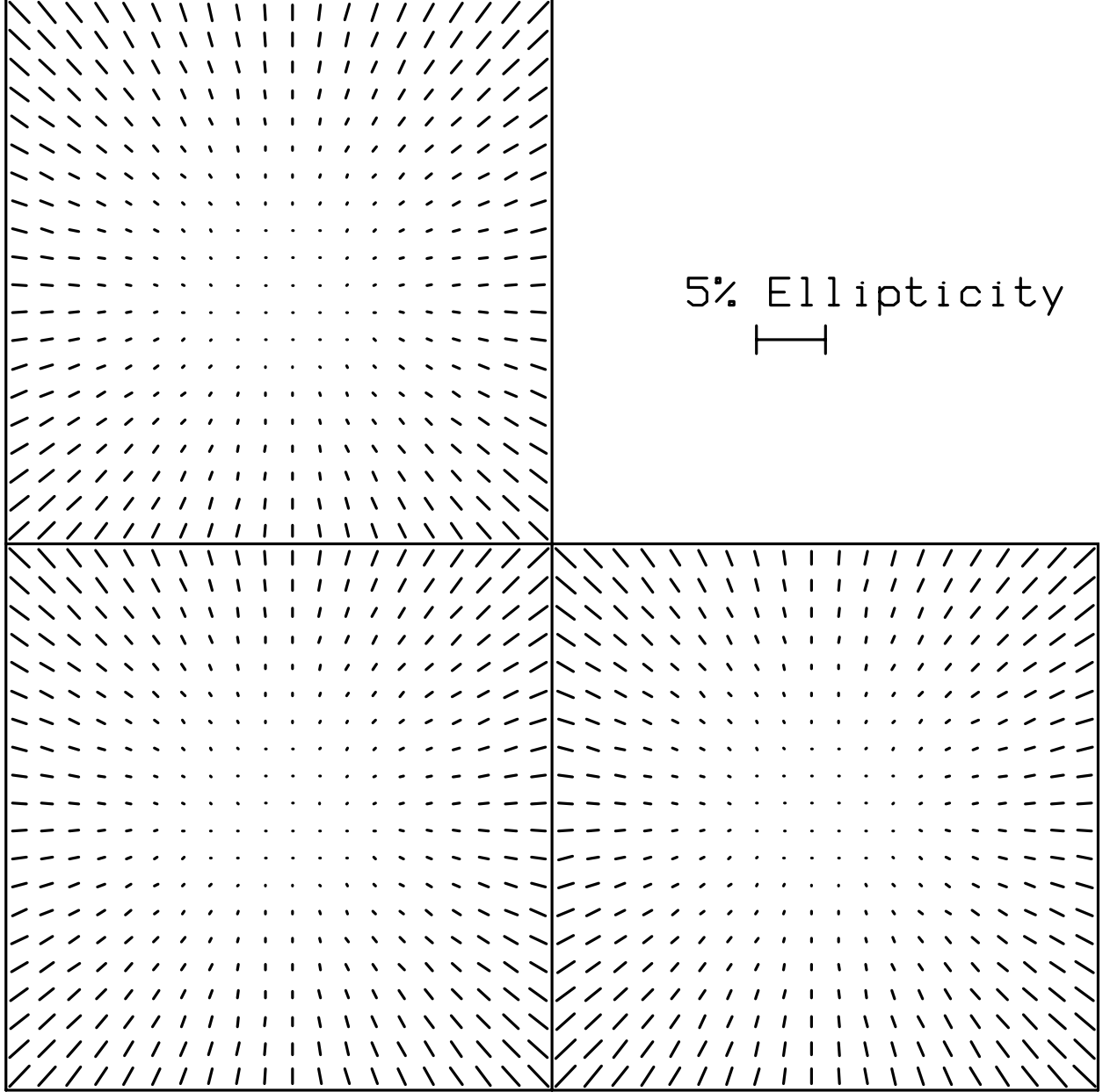
Fig. 3.— The WFPC2 Detector Shear pattern. The quantity plotted is \epsilon_i^\phi = 2\gamma_i which is the ellipticity induced by the detector shear for an intrinsically circular source. Chips 2, 3, and 4 are in the upper-left, lower-left, and lower-right corners, respectively. Chip 1 (the Planetary Camera) is not shown. Each chip is 1.3 arcmin on a side.
