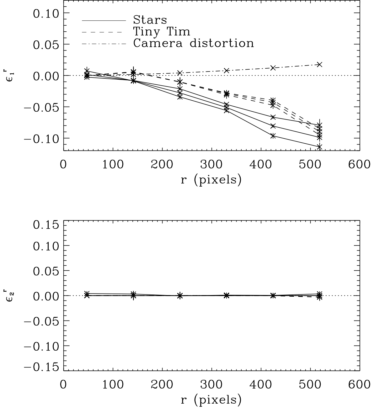
Fig. 7.— Rotated ellipticity profile for the PSF and the camera distortion, as a function of radius about the chip center. The solid lines show the ellipticity as measured for M4, combined M4/NGC6572, and NGC6572 stars, from top to bottom respectively. The dashed lines show the PSF ellipticity predicted by Tiny Tim for focus values of +2.0 , -1.5 , and -5.0\mu\text{m} , from top to bottom respectively. The dot-dashed line shows the distortion ellipticity \epsilon_i^\phi .
