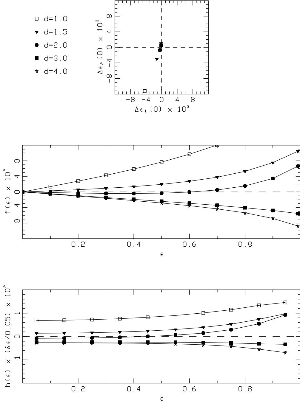
Fig. 2.— Residual errors of the PSF correction determined from numerical simulations. Panels (a), (b) show, respectively, the constant term \Delta\epsilon_i(0) and the radial function f(\epsilon) , for measuring absolute ellipticities. Panel (c) shows the radial function h(\epsilon) for measuring an ellipticity change of \delta\epsilon_i = 0.05 (see text). These quantities are plotted as a function of the unweighted galaxy ellipticity \epsilon and size d (in WPC2 pixels).
