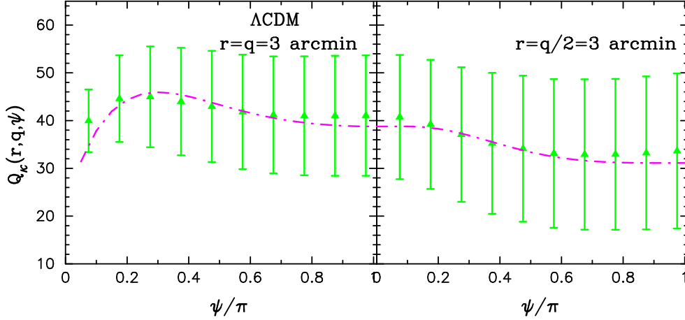
Figure 8. The reduced 3PCF of the convergence field, Q_\kappa , for the \Lambda CDM model against triangle configurations parameterized by r , q and \psi (see Figure 4). The left panel shows the result for isosceles triangles with r = q = 3' fixed and varying \psi , while the right panel for more elongated triangles with r = q/2 = 3' .
