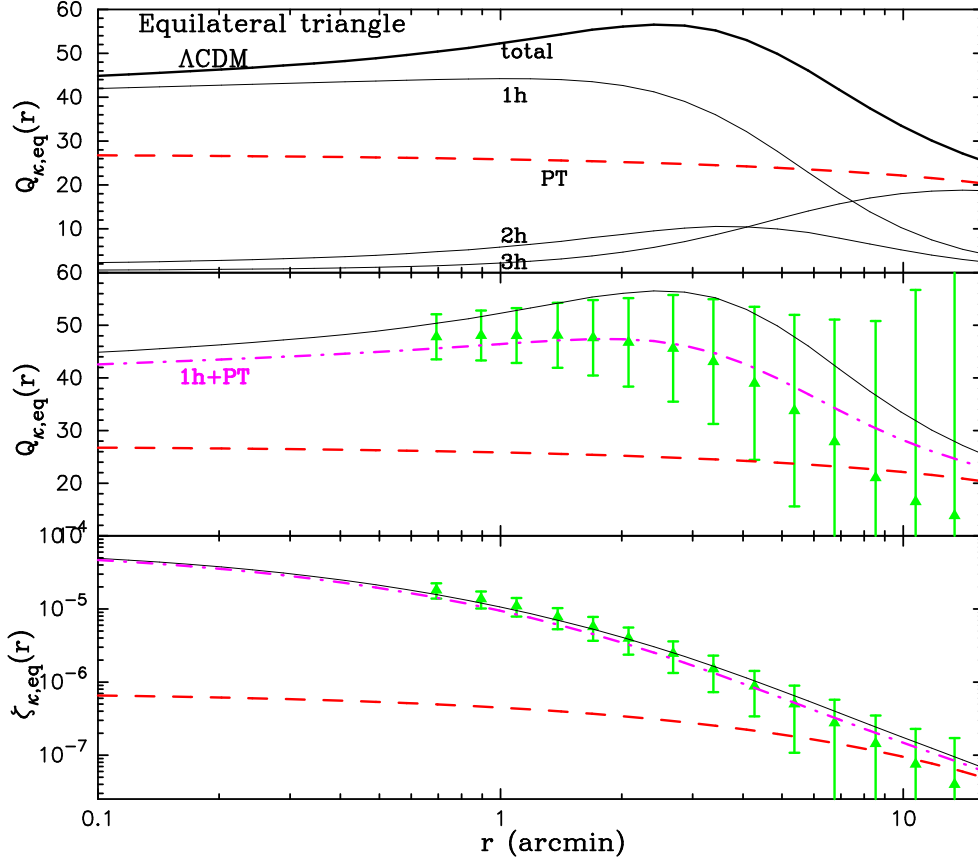
Figure 6. The 3PCF of the convergence field for equilateral triangles against side length r in arcminutes. Top panel: The thick solid curve shows the halo model prediction for the reduced 3PCF, Q_\kappa , defined by equation (37). The thin solid curves denote the 1-, 2- and 3-halo term contributions separately. The dashed curve is the perturbation theory (PT) prediction. Middle panel: The comparison with simulations for Q_\kappa , as in Figure 5. The simulation result does not display the bump in Q_\kappa seen in the halo model prediction. This is likely to be due to halo boundary effects in the standard implementation of the halo model (see text for details). The dot-dashed curve denotes the result if we replace the 2- and 3-halo terms with the PT prediction. This modified halo model agrees well with the simulation result. Bottom panel: The comparison for the 3PCF itself, as in the middle panel.
