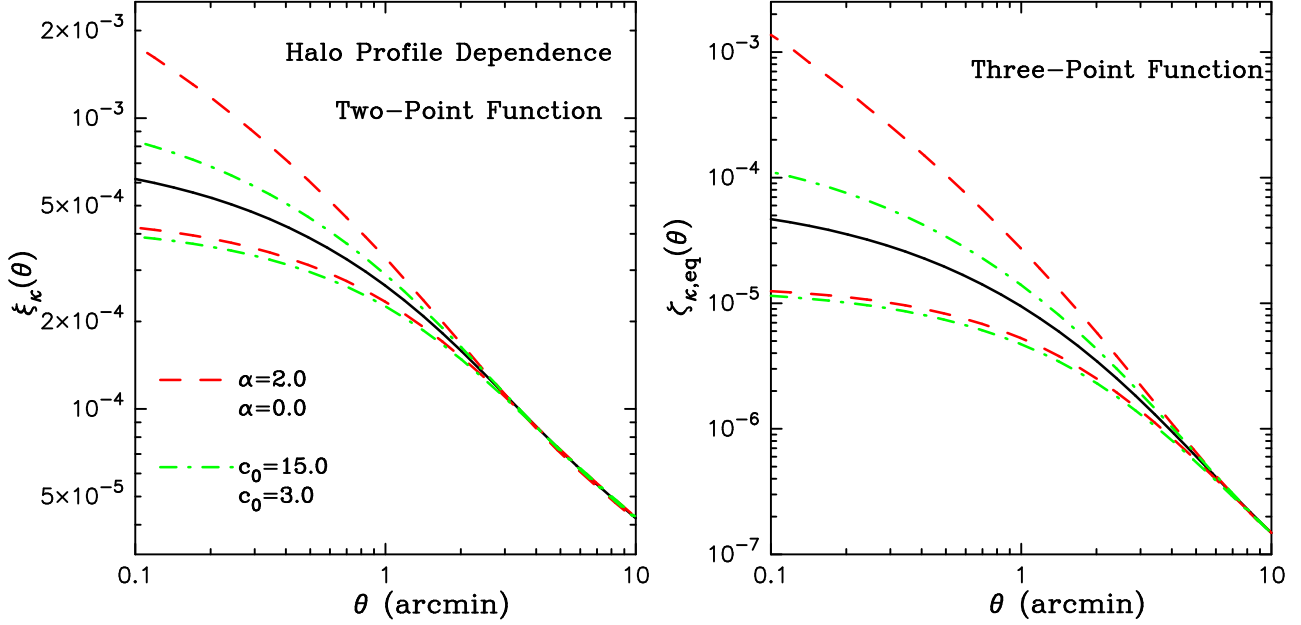
Figure 13. The dependences of the 2PCF (left panel) and 3PCF (right panel) of the convergence field on halo profile parameters. The upper and lower dashed curves show the halo model predictions with \alpha = 2 and 0 for the inner slope parameter of the generalized NFW profile of equation (10). The upper and lower dot-dashed curves are the results for the concentration parameter c_0 = 15 and 3. The solid curve is the halo model result for our reference model, the NFW profile with \alpha = 1, c_0 = 9 .
