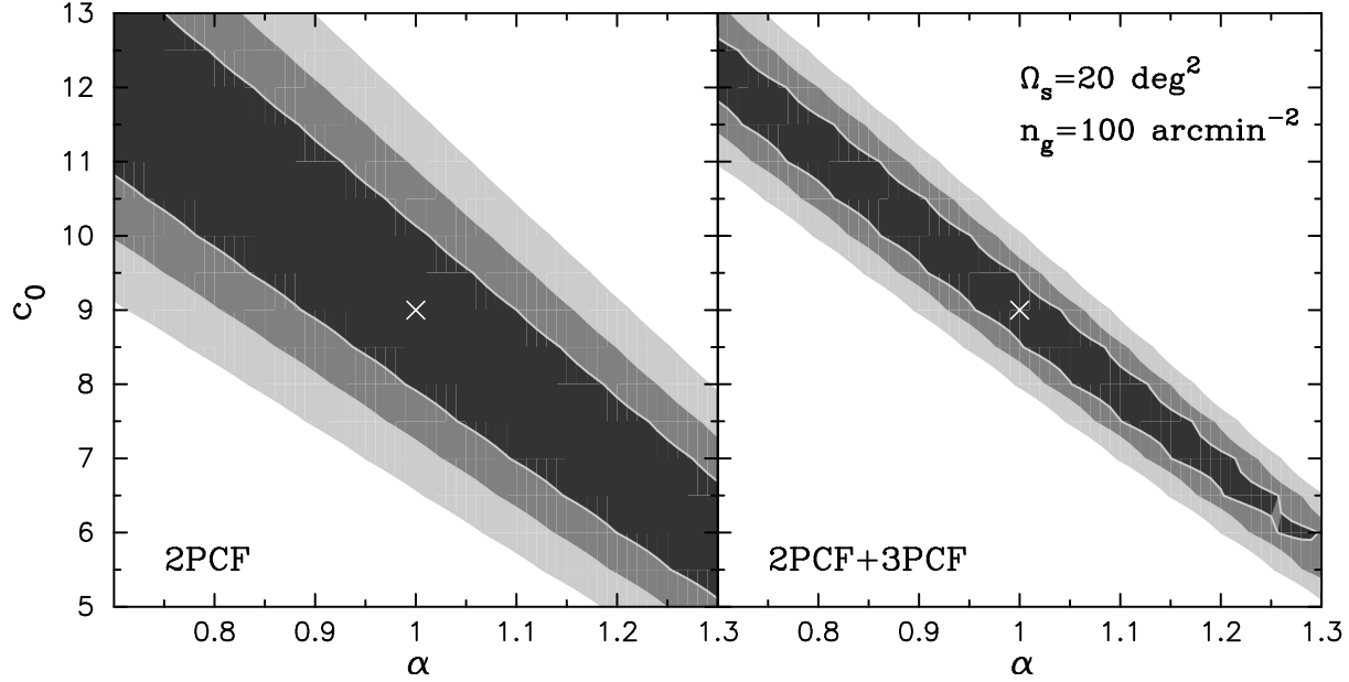
Figure 17. As in the previous figure, but for a survey with \Omega_s = 20 \text{ deg}^2 and n_g = 100 \text{ arcmin}^{-2} . The results show the value of increased number density of galaxies that can be achieved with a deeper survey. For such a survey the 3PCF provides a much larger improvement in the constraints.
