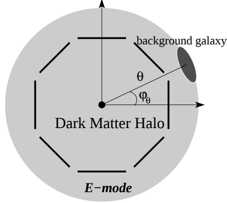
Figure 1. Illustration of the shear pattern around an axially-symmetric halo. A background galaxy image is tangentially deformed with respect to the halo center, corresponding to a pure E mode in the shear field.
