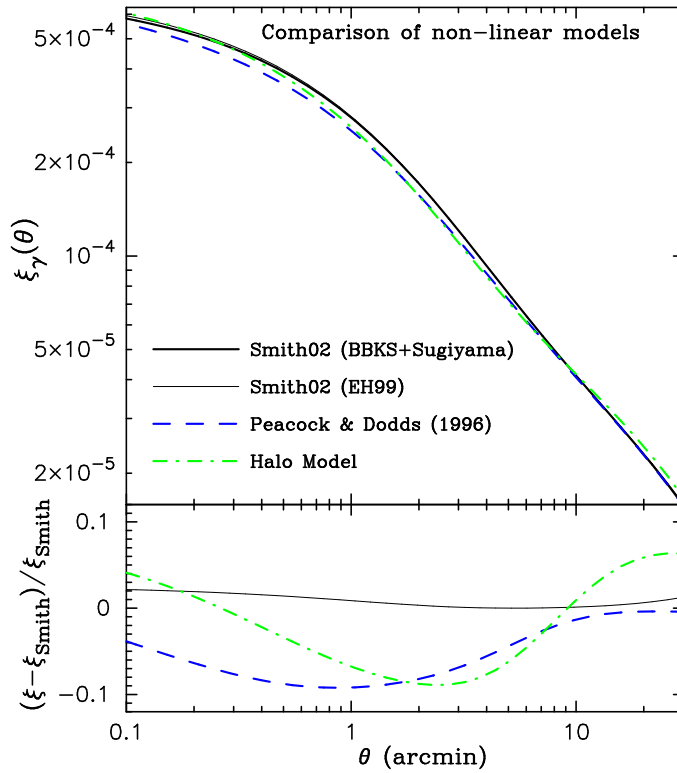
Figure A3. Comparison of model predictions for \xi_\gamma . The solid, dashed and dot-dashed curves are the results from the Smith02 formula, the PD formula and the halo model, respectively. The lower panel explicitly shows the deviation of each model prediction from the Smith02 model. Although all the results agree with each other within 10%, the Smith02 result for \xi_\gamma is higher than the PD result by 0 – 10% at 0.1 \lesssim \theta \lesssim 10' (see text for details). Note that the Smith02 result is computed using the BBKS transfer function. To demonstrate the effect of the input linear power spectrum, the thin solid curve is the Smith02 result when we use the fitting formula of Eisenstein & Hu (1999), which is more accurate.
