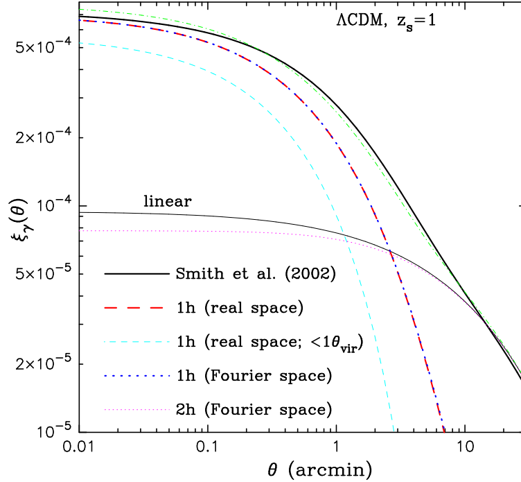
Figure A1. The two-point correlation function of the shear field, \xi_\gamma(\theta) = \langle \gamma \cdot \gamma^* \rangle , vs. separation angle \theta . The thick dashed curve shows the real-space halo model prediction for the 1-halo term, computed using equation (20), while the thick dotted curve shows the Fourier-space halo model prediction. The sum with the 2-halo term, denoted by the thin dotted curve, leads to the halo model prediction for the total power (1h+2h terms) shown by the dot-dashed curve. For comparison, the thick and thin solid curves show the predictions computed from the Smith02 fitting formula for the non-linear mass power spectrum and the linear power spectrum, respectively. The thin dashed curve is the real-space halo model prediction when the integration range is confined to the virial radius.
