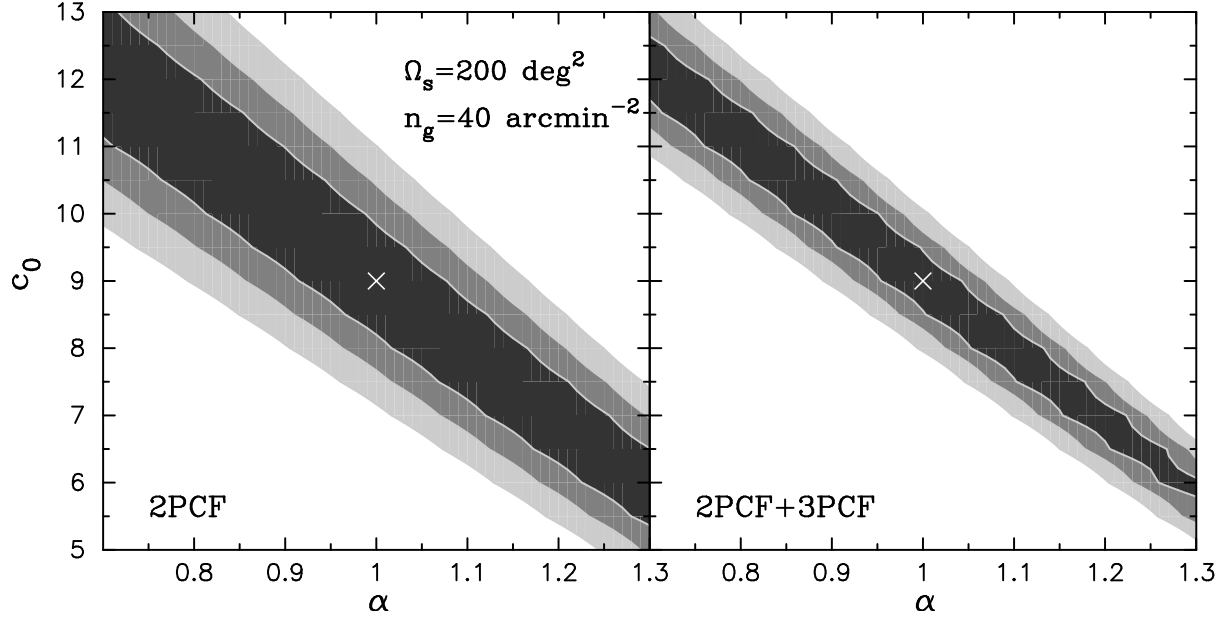
Figure 16. Contour plots of the constraints on the inner slope parameter \alpha and the halo concentration c_0 expected from a survey with area \Omega_s = 200 degree 2 and n_g = 40 arcmin -2 . The left panel shows the result if we use only the 2PCF measurement, while the right panel shows the result from combined measurements of the 2PCF and 3PCF. The cross symbol denotes input fiducial model of (\alpha, c_0) = (1.0, 9.0) . To perform the fitting, we have used measurements on scales [0.2, 2'] and combined 250 triangle configurations for the 3PCF (see text for details). The three shaded regions represent \Delta\chi^2 = 2.30(68.3\%) , 6.17(95.4\%) and 11.8(99.7\%) , respectively. The 3PCF measurement can tighten the constraints, reflecting the fact that it carries lensing information complementary to the 2PCF.
