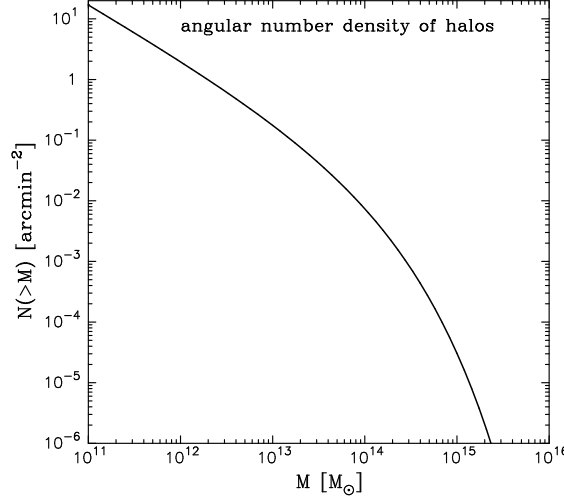
Figure 3. Projected number density of halos more massive than a given mass scale M , N(> M) , between z = 0 and 1 for the \Lambda CDM model.
