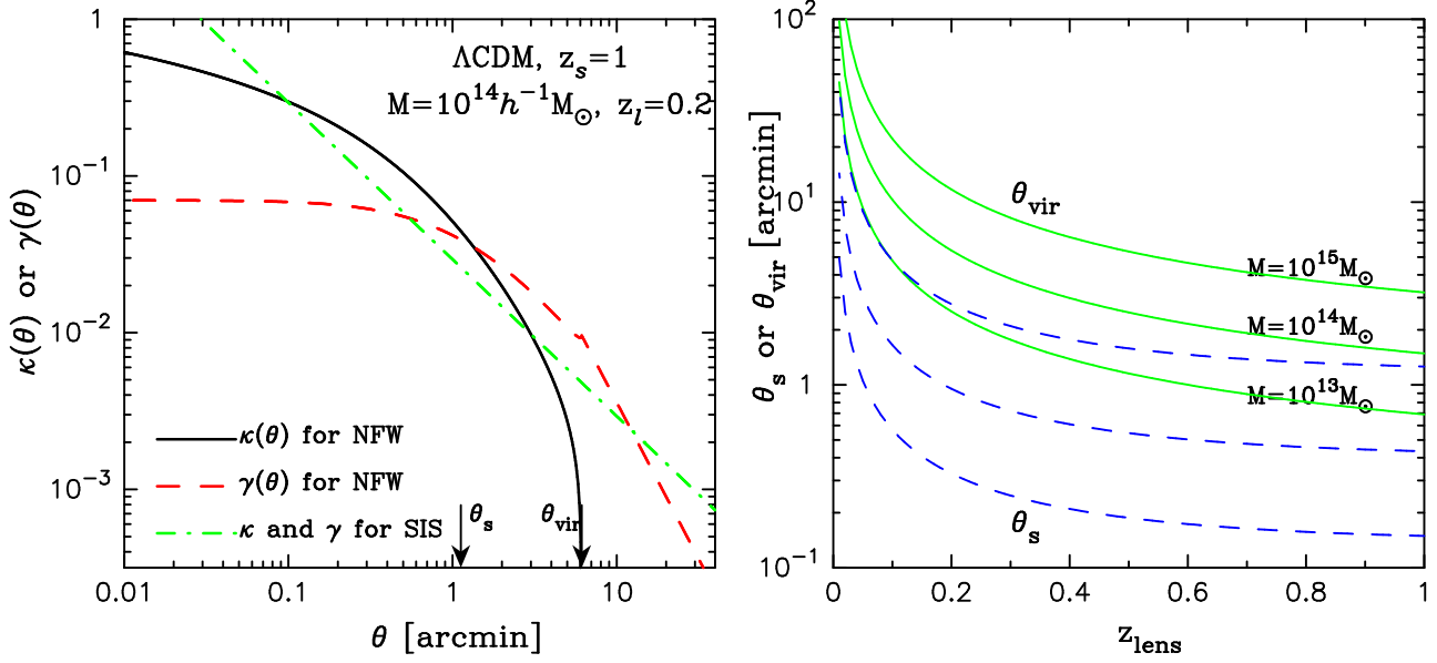
Figure 2. Left panel: Radial profiles of the convergence (solid curve) and shear (dashed curve) fields for an NFW halo. The halo mass is M = 10^{14} h^{-1} M_{\odot} , lens redshift z_l = 0.2 and source redshift z_s = 1 . For comparison, the dot-dashed curve shows a singular isothermal sphere ( \rho_h \propto r^{-2} ) with the same virial mass. The two arrows show the scale radius and the virial radius of the NFW profile. Right panel: The angular scales of the scale and virial radii for a lens halo are plotted against its redshift. The three curves show the results for halo masses M/M_{\odot} = 10^{13}, 10^{14} and 10^{15} , from bottom to top. Halos relevant for lensing statistics have \theta_s \lesssim 2' for their scale radii at redshift z = 0.4 . Thus the effect of the inner structures of the halo profile on lensing statistics should appear at scales \lesssim 2' .
