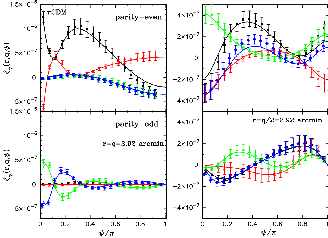
Figure 12. As in the previous figure, for the \tau CDM model. The cosmological parameters for the \tau CDM model are the same as for the SCDM model, except for the shape parameter \Gamma which is 0.21, while it is 0.5 for SCDM.
