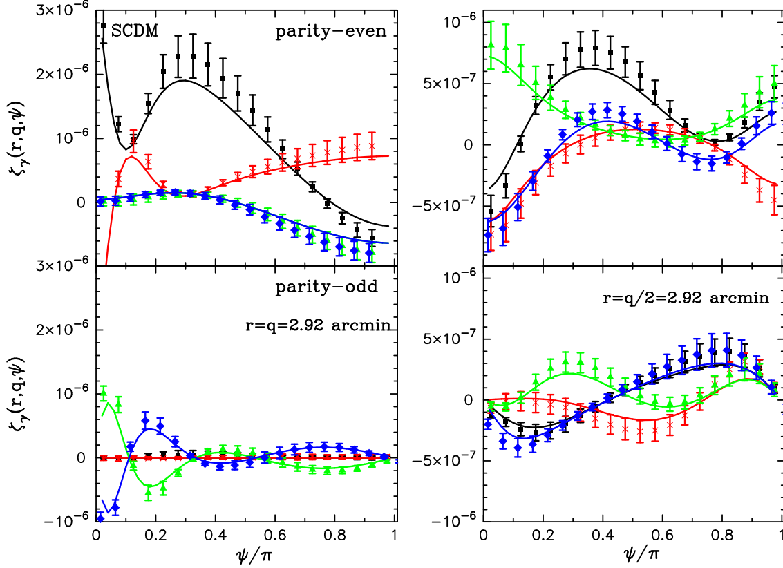
Figure 11. As in the previous figure, for the SCDM model.
