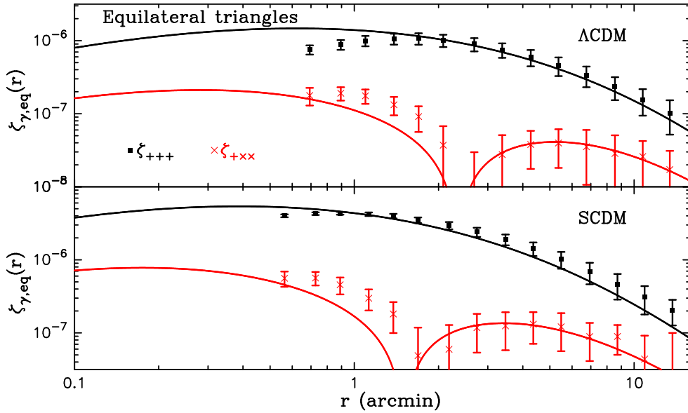
Figure 9. The shear 3PCFs for equilateral triangles against side length r for the \Lambda CDM (upper panel) and SCDM (lower panel) models, as in the bottom panel of Figure 6. From symmetry considerations, the four parity-odd functions defined by equation (32) vanish for an E -mode, and three of the parity even functions are equal. Hence, only the results for \zeta_{+++} and \zeta_{+xx} are shown. Note that the absolute value of \zeta_{+xx} is plotted, since it becomes negative at large scales. The two solid curves are the halo model predictions, using only the 1-halo term.
