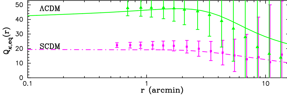
Figure 7. Plots for the SCDM model, as the middle panel in Figure 6. The square symbols show the simulation result for Q_\kappa for the SCDM model. The triangles denote the simulation results for the \Lambda CDM model, with the error bars scaled to the same area. The comparison shows the sensitivity of Q_\kappa to the cosmological model, in particular to \Omega_{m0} .
