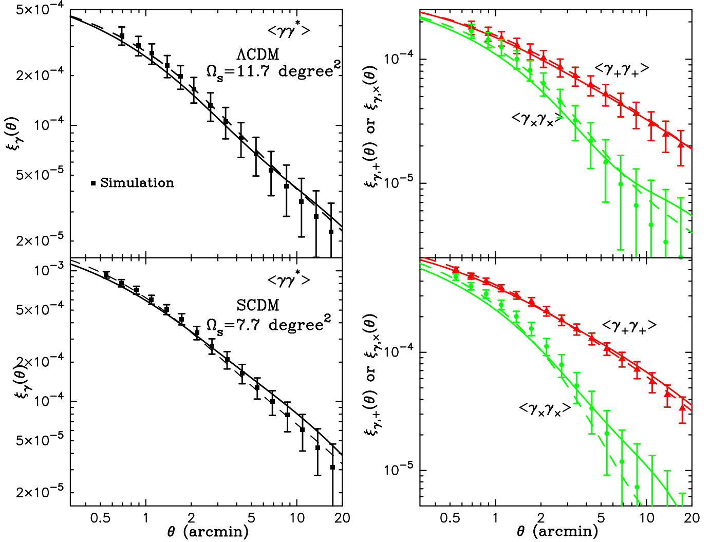
Figure 5. Comparison of model predictions for the shear 2PCFs with measurements from the ray-tracing simulations. The left panel shows the shear 2PCF, \xi_\gamma = \langle \gamma \cdot \gamma^* \rangle , for the \Lambda CDM (upper panel) and SCDM (lower panel) models. The solid and dashed curves are the predictions from the halo model and the Smith02 formula, respectively, while the square symbols with error bars denote the simulation result. Note that errors in different bins are highly correlated with each other. Similarly, the right panel shows the comparison for \xi_{\gamma,+} and \xi_{\gamma,\times} .
