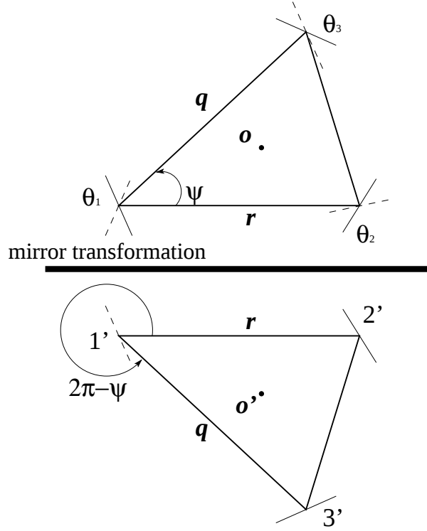
Figure 4. Upper: A sketch of the triangle configuration, parameterized by r , q and \psi , used to describe the 3PCF. The solid and dashed lines at each vertex show the positive directions of the + and \times components of the shear field, defined with respect to the triangle center denoted by o . Lower: The mirror transformation of the triangle with respect to the side vector r for \xi_{\times++} is shown as one example. The \gamma_{\times} component at each vertex changes sign under the mirror transformation (at vertices 1 and 1' in this case).
