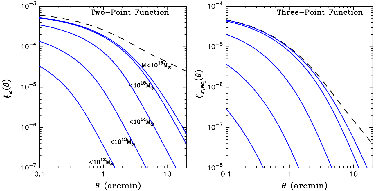
Figure 14. The dependences of the 1-halo term contribution to the convergence 2PCF (left panel) and 3PCF (right panel) on the maximum mass cutoff used in the calculation. From top to bottom, the five solid curves are the results for a maximum mass of 10^{16} , 10^{15} , 10^{14} , 10^{13} and 10^{12} M_\odot , as indicated. The dashed curve shows the total halo model prediction. Most contributions arise from halos of M > 10^{13} M_\odot on the scales we have considered, and the 3PCF is more sensitive to massive halos than the 2PCF.
