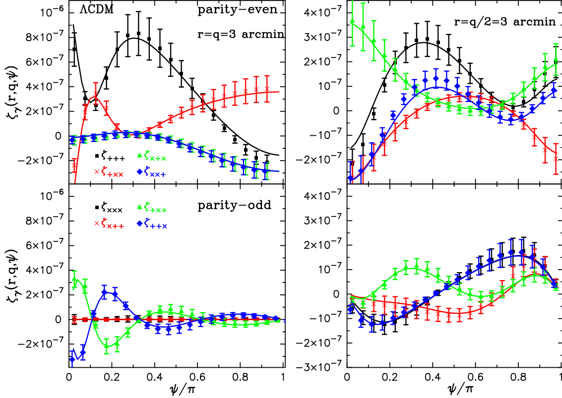
Figure 10. The eight shear 3PCFs for the \Lambda CDM model against triangle configurations, as in Figure 8. The upper and lower plots show the results for the parity-even and -odd functions, respectively. Note that range on the y-axis for the right panel is about two times smaller than in the left panel. The solid curves show the halo model predictions for the eight shear 3PCFs, while the symbols are the simulation results as indicated.
