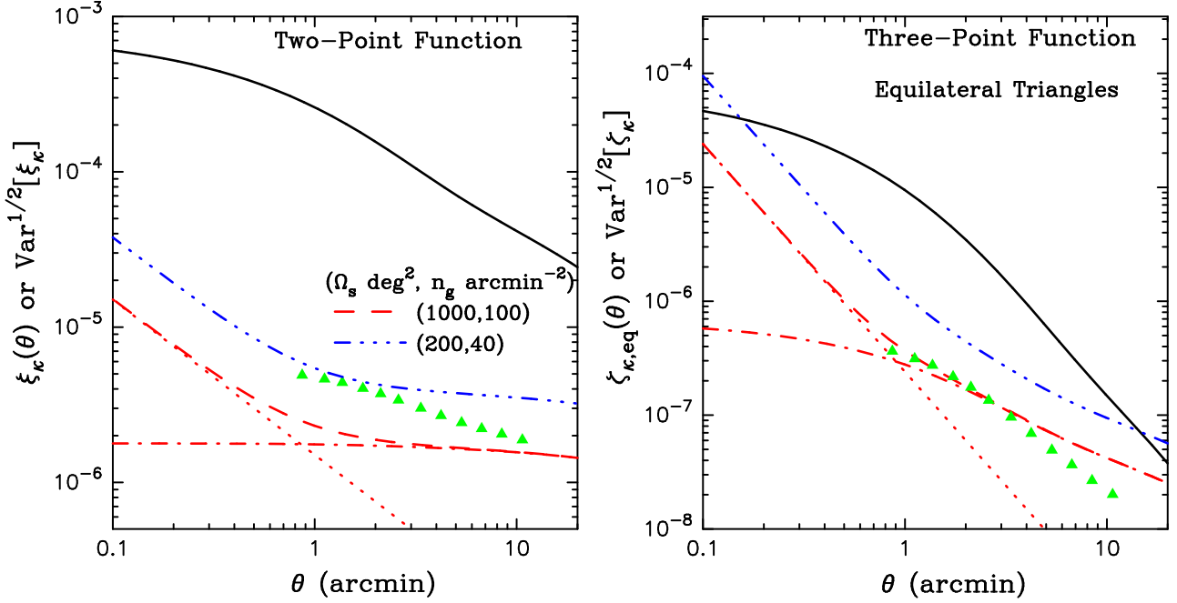
Figure 15. Error estimates for measurements of the convergence 2PCF (left panel) and 3PCF (right panel) for the \Lambda CDM model. The error estimate includes both the shot noise due to intrinsic ellipticities, with rms \sigma_e = 0.4 , and sample variance. Two cases for survey area \Omega_s and number density of source galaxies n_g are shown. For (\Omega_s, n_g) = (1000 \text{ deg}^2, 100 \text{ arcmin}^{-2}) , the dotted and dot-dashed curves show the shot noise contribution and the sample variance separately: shot-noise dominates on sub-arcminute scales. The solid curve shows the halo model prediction for the 2PCF or the 3PCF. The triangular symbols show the sample variance estimated from simulations for \Omega_s = 1000 .
