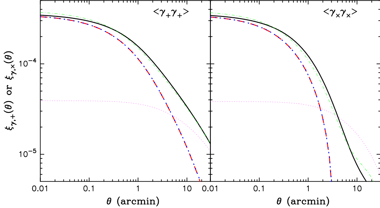
Figure A2. The two-point correlation functions of the shear fields, \xi_{\gamma,+} (left panel) and \xi_{\gamma,\times} (right panel), as in Figure A1. Although the 2-halo term for \xi_{\gamma,\times} overestimates the amplitude at large scales \theta \gtrsim 5' , the halo model reproduces the Smith02 result because the 1-halo term is negative.
