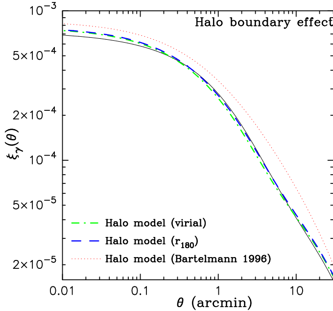
Figure A4. The figure shows how the halo boundary condition employed in the halo model calculation affects the prediction for \xi_\gamma . The thick dot-dashed and dashed curves are the results when we employ the NFW profile truncated at the virial radius and at the radius r_{180} , respectively. The radius r_{180} is defined so that mean density enclosed by a sphere with radius r_{180} is 180 times the background density. The upper dotted curve shows the halo model prediction if one uses the expression in Bartelmann (1996) for the shear profile to compute the 1-halo term. For reference, the thin solid curve shows the Smith02 result in Figure A1.
