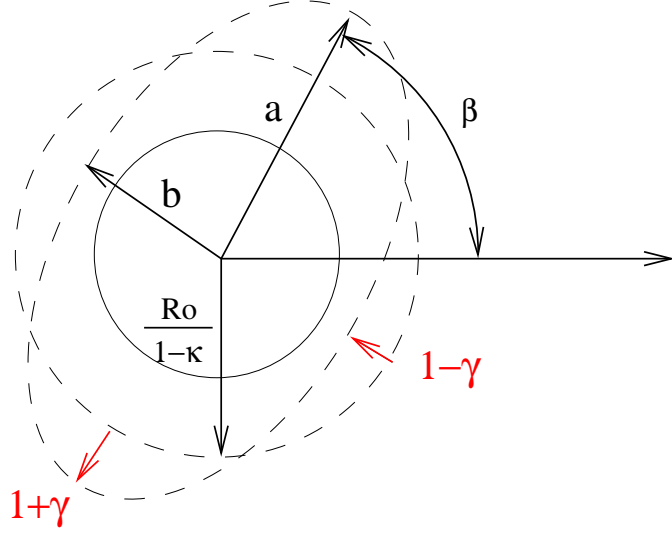
Figure 3. Illustration of the first order effect of cosmic shear on a circular background galaxy of radius R_0 . The convergence is an isotropic distortion of the image of the galaxy, while the shear is an anisotropic distortion.
