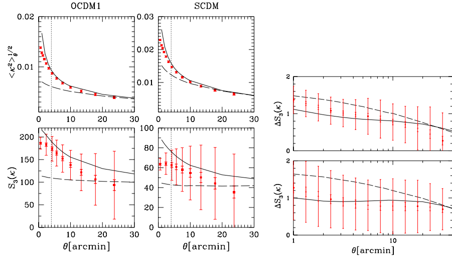
Figure 26. Left panel: variance and skewness of the top-hat smoothed convergence field a OCDM ( \Omega_0 = 0.3 , \sigma_8 = 0.85 , z_s = 1.03 , \Gamma = 0.21 ) and SCDM model ( \Omega_0 = 1. , \sigma_8 = 0.6 , z_s = 1.03 , \Gamma = 0.5 ). The solid lines show the non-linear predictions, and the dashed lines the leading order of the perturbation theory calculations. The vertical dotted lines in the left panels denote the reliable scale limit fixed by the resolution of the ray-tracing simulation. The “large” error bars correspond to a survey of 25 square degrees, and the small error bars to 1000 square degrees. Right panel: Skewness correction due to the Born approximation and lens-lens coupling for SCDM (top) and OCDM1 (bottom) measured in ray-tracing simulation.
