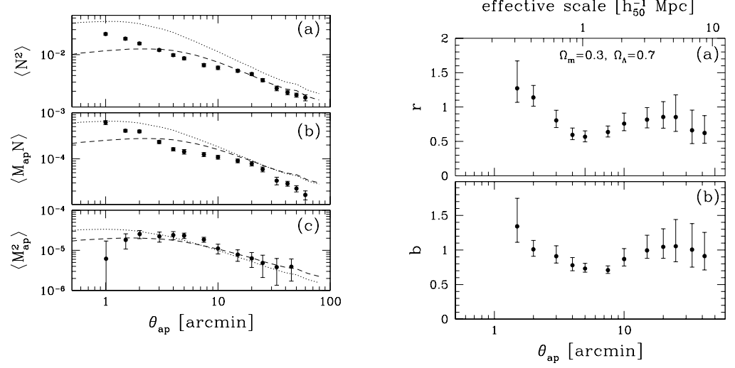
Figure 23. Left plot: The measurements of \langle \mathcal{N}^2 \rangle (panel a), and \langle \mathcal{N} M_{\text{ap}} \rangle (panel b) as a function of angular scale from the RCS data. Panel c shows \langle M_{\text{ap}}^2 \rangle as a function of angular scale from the VIRMOS-DESCART data. The error bars for \langle M_{\text{ap}}^2 \rangle have been increased to account for the unknown correction for the observed “B”-mode. For reference, a few models have been plotted, assuming b = 1 and r = 1 , for an OCDM cosmology (dotted line; \Omega_m = 0.3 , \Omega_\Lambda = 0 , \sigma_8 = 0.9 , and \Gamma = 0.21 ) and a \Lambda CDM cosmology (dashed line; \Omega_m = 0.3 , \Omega_\Lambda = 0.7 , \sigma_8 = 0.9 , and \Gamma = 0.21 ). Note that the points at different scales are only slightly correlated. Right plot: The measured value of the galaxy-mass cross correlation coefficient r as a function of scale for the \Lambda CDM cosmology. (b) The bias parameter b as a function of scale. The upper axis indicates the effective physical scale probed by the compensated filter at the median redshift of the lenses ( z = 0.35 ).
