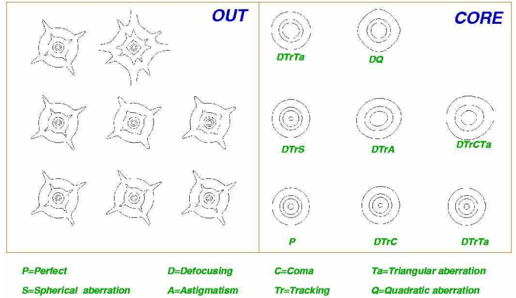
Figure 10. Right plots: simulated cores of anisotropic PSF's. Left plots: simulated outer part of the PSF (Erben et al. 2001). The different PSFs are computed from ray-tracing through the telescope optic.
