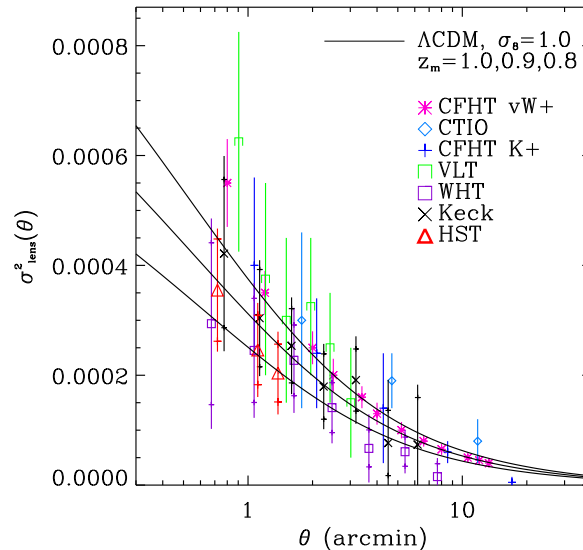
Figure 15. Compilation of recent results of top-hat shear variance measurements from several groups (Courtesy Réfrégier et al. 2002).
