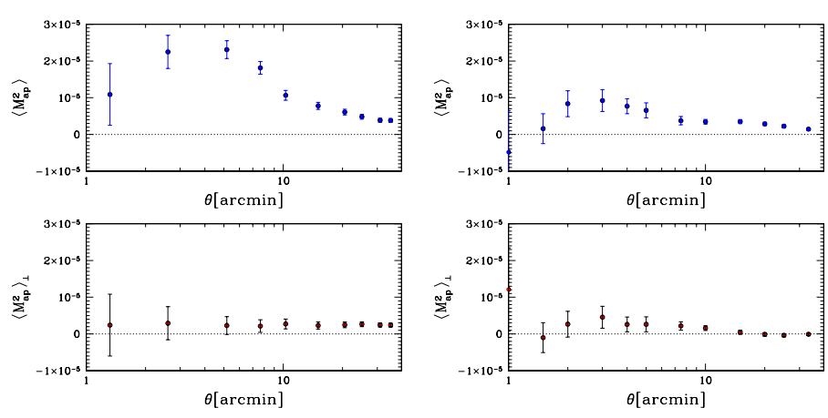
Figure 17. Left: E (top) and B (bottom) modes measured with all the most recently reduced data in the VIRMOS survey (Van Waerbeke et al. 2002). Right: E (top) and B (bottom) modes measured in the RCS survey (Hoekstra et al. 2002). The B mode is low and the E mode compatible with the predictions for the aperture mass statistics.
