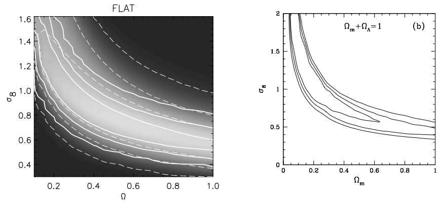
Figure 19. The solid lines on each plot show the 1, 2 and 3\sigma contours of the VIRMOS and RCS survey, from the measurements shown in Figure 17. The contours have been marginalised over the source redshift and the slope of the matter power spectrum as described elsewhere (Van Waerbeke et al. 2002, Hoekstra et al. 2002).
