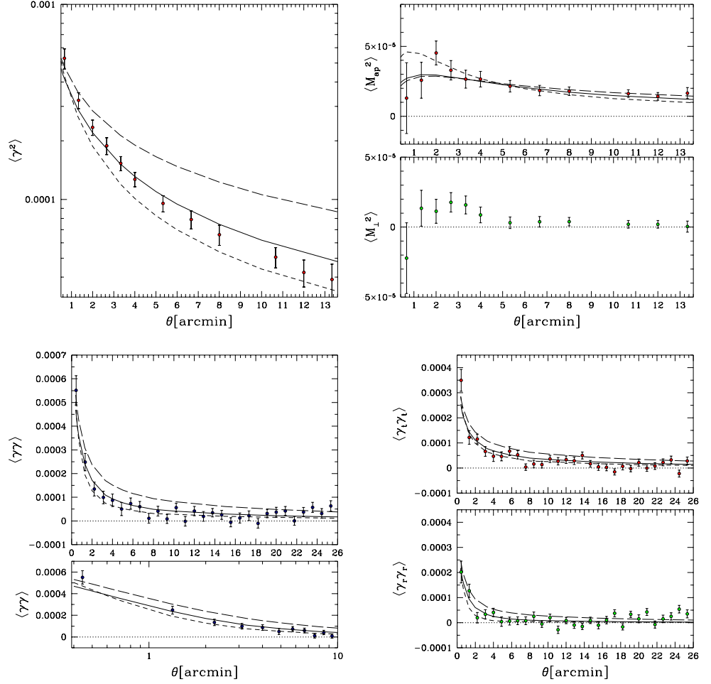
Figure 16. Measurement of all the 2-points statistics in the same survey, VIRMOS (Van Waerbeke et al. 2001). Top left: top-hat variance. Top right: aperture mass E and B modes. Bottom left: full shear correlation function. Bottom right: projected shear correlation functions. survey. Right: E (top) and B (bottom) modes measured in the RCS survey. The B mode is low and the E mode compatible with the predictions for the aperture mass statistics. The lines are fiducial models which indicate the relative deviations between the statistics to the models.
