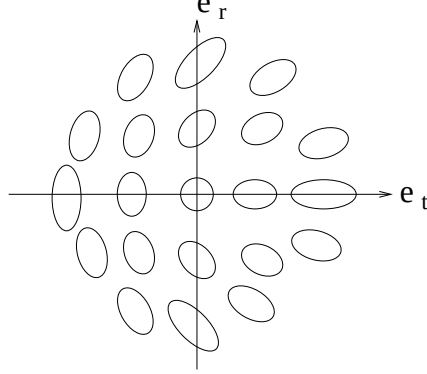
Figure 12. Value of (e_t, e_r) , or (e_1, e_2) in Cartesian coordinates, as a function of the shape of a galaxy with respect to the local frame attached to the galaxy. Note that the ellipticity is invariant by a rotation of \pi , and not 2\pi , this is why e_t < 0 and e_r = 0 for a vertical galaxy for instance.
