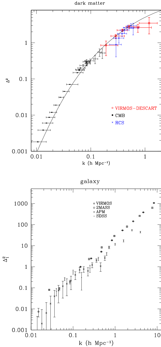
Figure 24. Top: Dark matter 3D power spectrum, deprojected from the 2D convergence power spectrum measured in the VIRMOS survey, using SVD (Pen et al. 2003). The power is rescaled to z = 0 , points are compared to the CMB (WMAP) and RCS lens survey. Bottom: Galaxy 3D power spectrum deprojected using the same method. For comparison, points from 2MASS, APM and SDSS are also shown.
