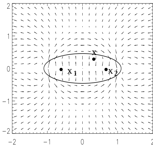
Figure 20. Average shear pattern obtained around a galaxy pair located at (\mathbf{x}_1, \mathbf{x}_2) . A third galaxy is located at \mathbf{x} , its shear vector is projected along the vertical axis, it is called \gamma_t(\mathbf{x}) . The shear 3-points function \langle \gamma(\mathbf{x}_1) \cdot \gamma(\mathbf{x}_2) \gamma_t(\mathbf{x}) \rangle is averaged inside the ellipse indicated by the solid line.
