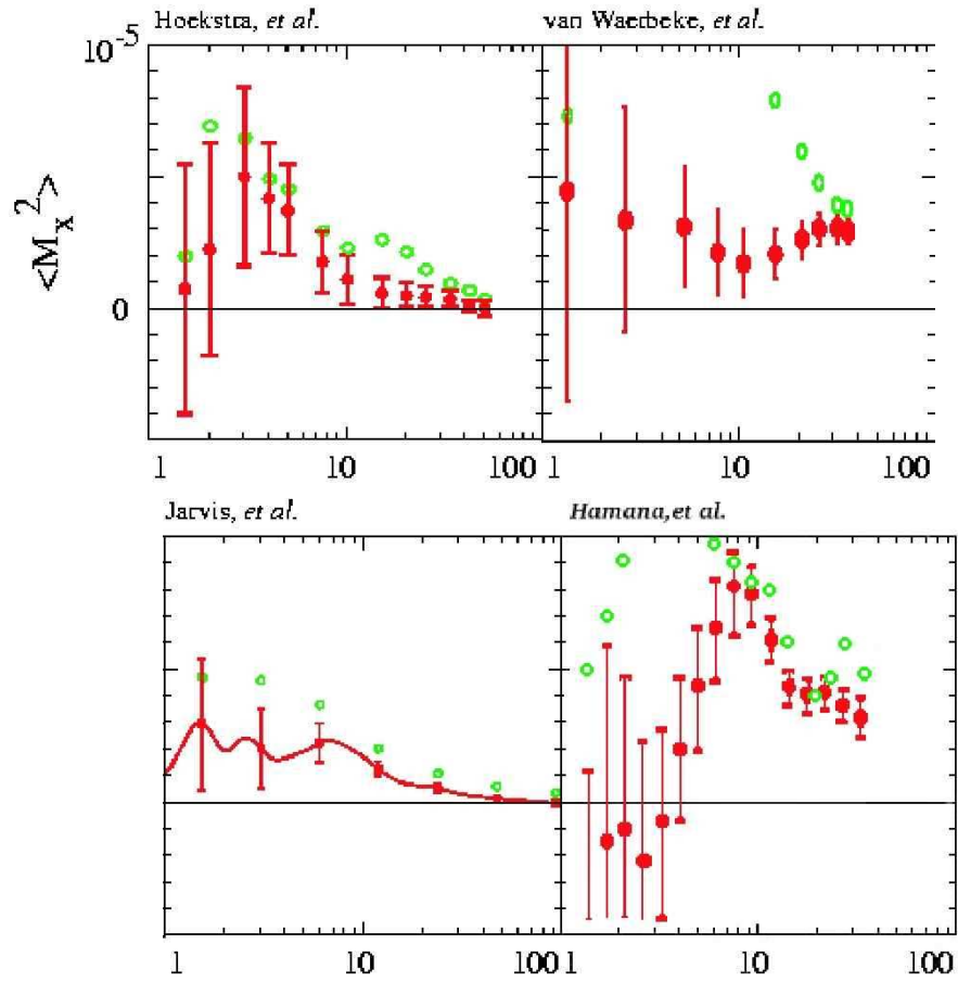
Figure 18. Plot showing the relative amplitude of the aperture mass E and B modes (points without and with error bars respectively) for all the surveys where the aperture mass has been measured (Hoekstra et al. 2002, Van Waerbeke et al. 2002, Jarvis et al. 2003 and Hamana et al. 2003) (picture taken from Jarvis et al. 2003 and extended). The result of Hoekstra et al. (2002) is for the full magnitude range, while in Figure 17, right panel, it is for the galaxies used for the cosmic shear analysis.
