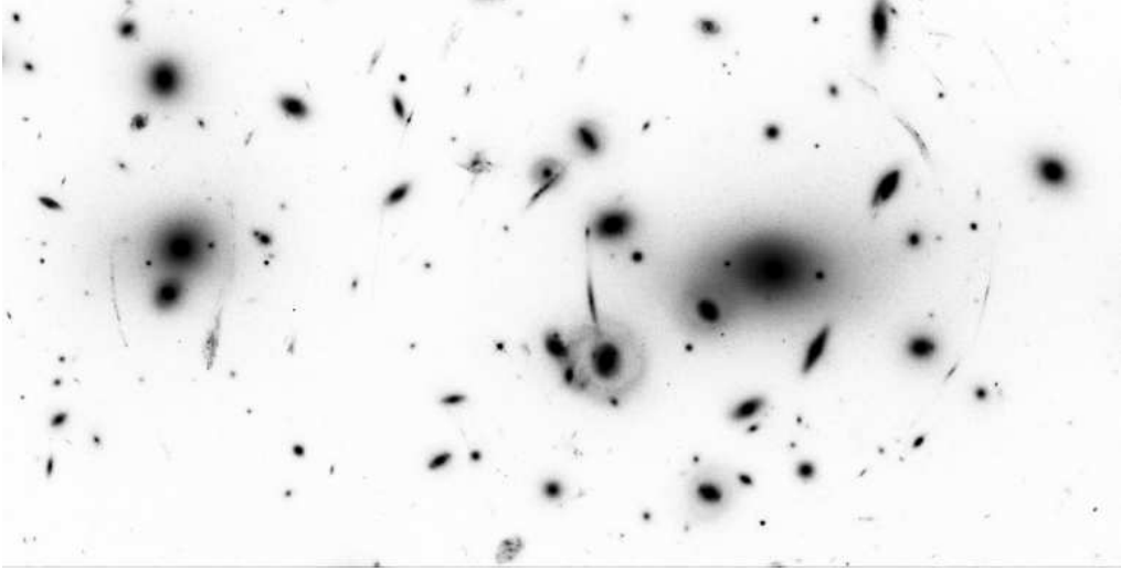
Figure 23: Hubble Space Telescope image of the cluster Abell 2218, showing a number of arcs and arclets around the two centers of the cluster. (NASA HST Archive)
