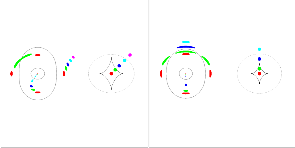
Figure 19: Compact source moving away from the center of an elliptical lens. Left panel: source crossing a fold caustic; right panel: source crossing a cusp caustic. Within each panel, the diagram on the left shows critical lines and image positions and the diagram on the right shows caustics and source positions.
