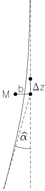
Figure 3: Light deflection by a point mass. The unperturbed ray passes the mass at impact parameter b and is deflected by the angle \hat{\alpha} . Most of the deflection occurs within \Delta z \sim \pm b of the point of closest approach.
