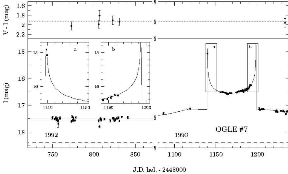
Figure 11: Light curve of the first binary microlensing event, OGLE #7 (taken from the OGLE WWW home page at http://www.astrouw.edu.pl/~ftp/ogle/ogle.html ).
