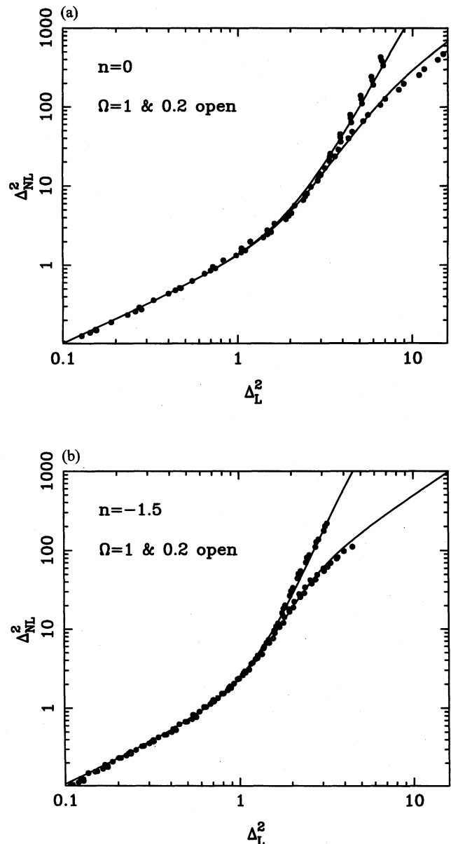
Figure 2. The generalized HKLM function relating non-linear power to linear power, for \Omega_m=1 and 0.2 at zero vacuum energy. (a) An n=0 spectrum; (b) n=-1.5 . The solid lines show the fitting formula of Section 3.3. As \Omega decreases, the non-linear power increases and the quasi-linear portion steepens. However, these changes are largely associated with the increase of f_{NL} in the virialized regime with \Delta_{NL}^2 \gtrsim 100 .
