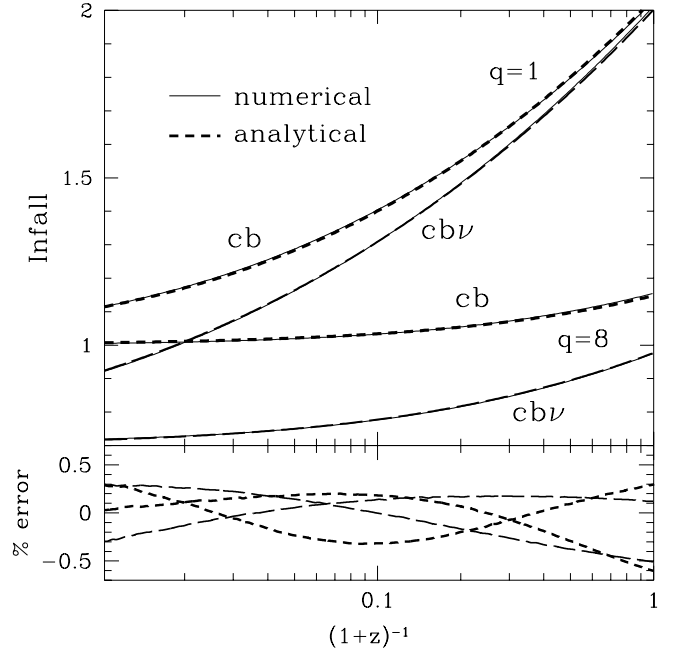
FIG. 2.—Analytic vs. numerical descriptions of neutrino infall for f_v = 0.3, f_b = 0.01, \Omega_0 = 1, h = 0.5 . Upper panel: Growth functions compared to the fully free-streaming time dependence of y^{1-p_{cb}} ; the case without infall is represented by a horizontal line of amplitude 1 ( cb ) and f_{cb} = 0.69 ( cbv ) here. Numerical CDM plus baryon fluctuations are compared with growth function D_{cb} (short-dashed lines) and numerical CDM plus baryon plus neutrino density-weighted fluctuations with D_{cbv} (long-dashed lines). Lower panel: Relative error.
