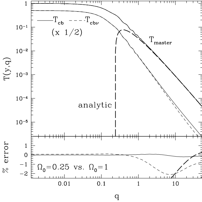
FIG. 4.—Demonstration of the invariance of the master function ( T_{\text{master}} ) under changes in the cosmological constant \Lambda . The model has the same \Omega_0 h^2, f_b , and f_v as Fig. 3 at z = 0 , but with \Omega_0 = 0.25 . Division of T_{cb} and T_{cbv} by the growth functions returns the master function T_{\text{master}} over which the estimate of Fig. 3 and the small-scale analytic solution are plotted (upper panel). The errors are plotted relative to T_{\text{master}} from the T_{cb} , z = 0 estimate of Fig. 3 and show agreement at the 1%–2% level (lower panel).
