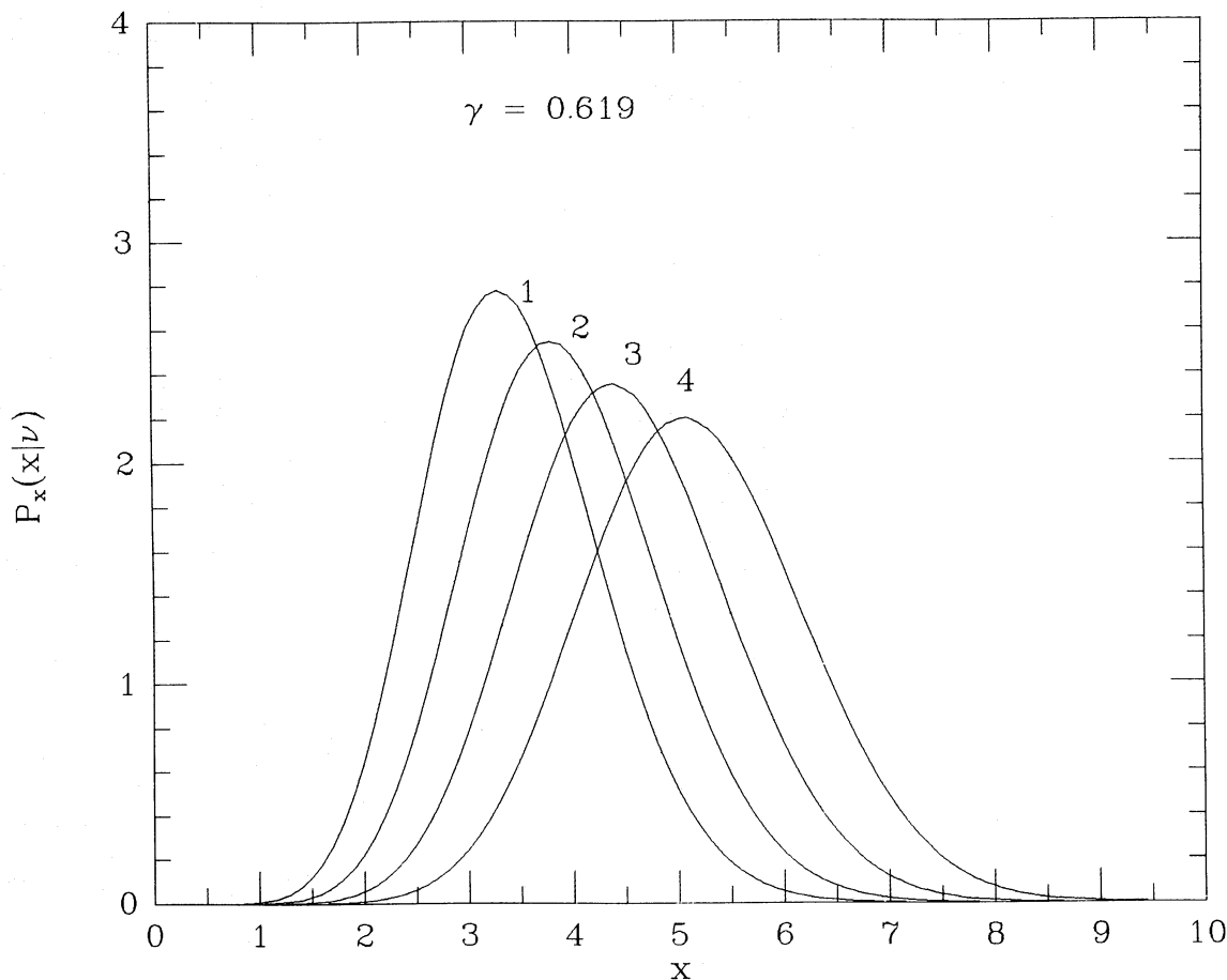
FIG. 6.—The constrained probability P(x|v) of eq. (7.5) giving the distribution of x = -\nabla^2 F/\sigma_2 for peaks. (The x used here is 1.58 times that in the text.)
