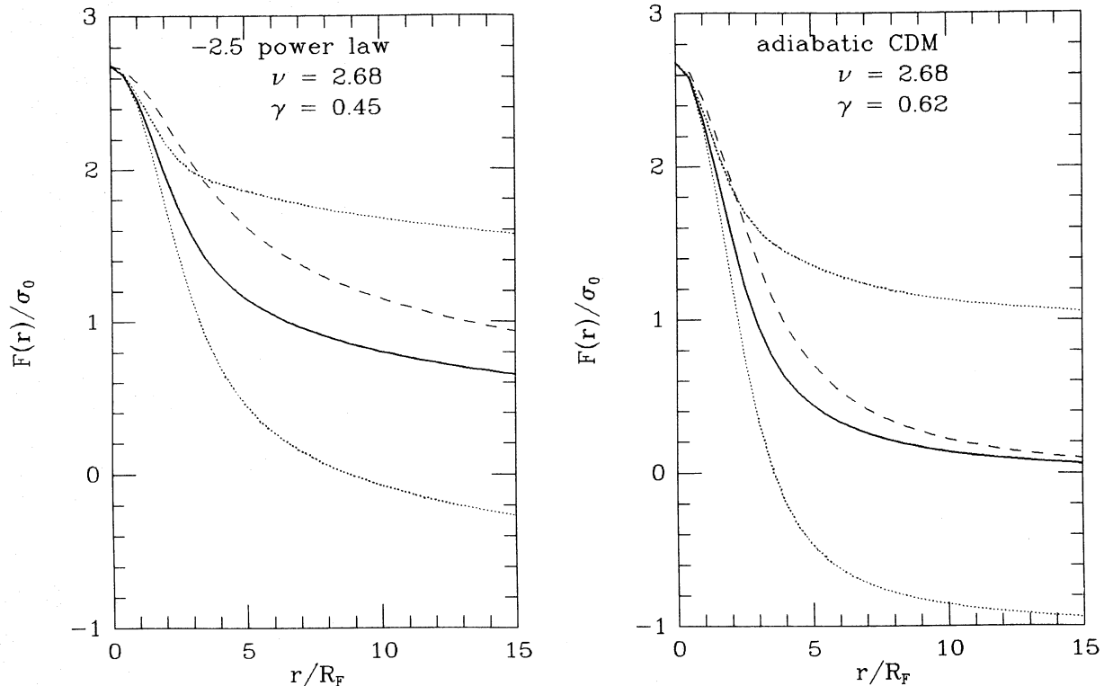
FIG. 8.—Orientation-averaged density profile about a peak of height \nu = 2.7 and its \pm 1 \sigma deviations are compared with the average profile for an ambient field point. Parameters are typical of CDM models of galactic scale structure. The mean spacings of peaks filtered on this scale in units of R_f for the n = -2.5 and adiabatic examples, respectively, are 18 and 13 for \nu > 2.68 ; 7.5 and 6.3 for \nu > 1 , which is also just about the spacing for peaks of arbitrary height.
